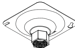
AI CPSPS
