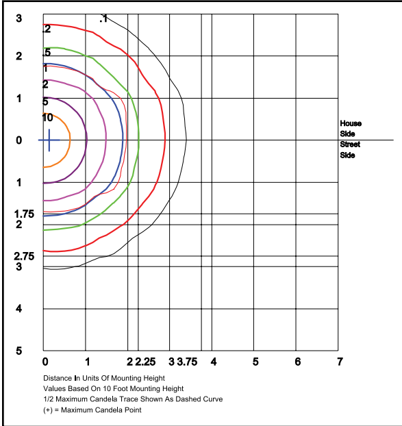
AIKH45QF1X167UAMC- Type V Grid in MH MH=10 Feet
